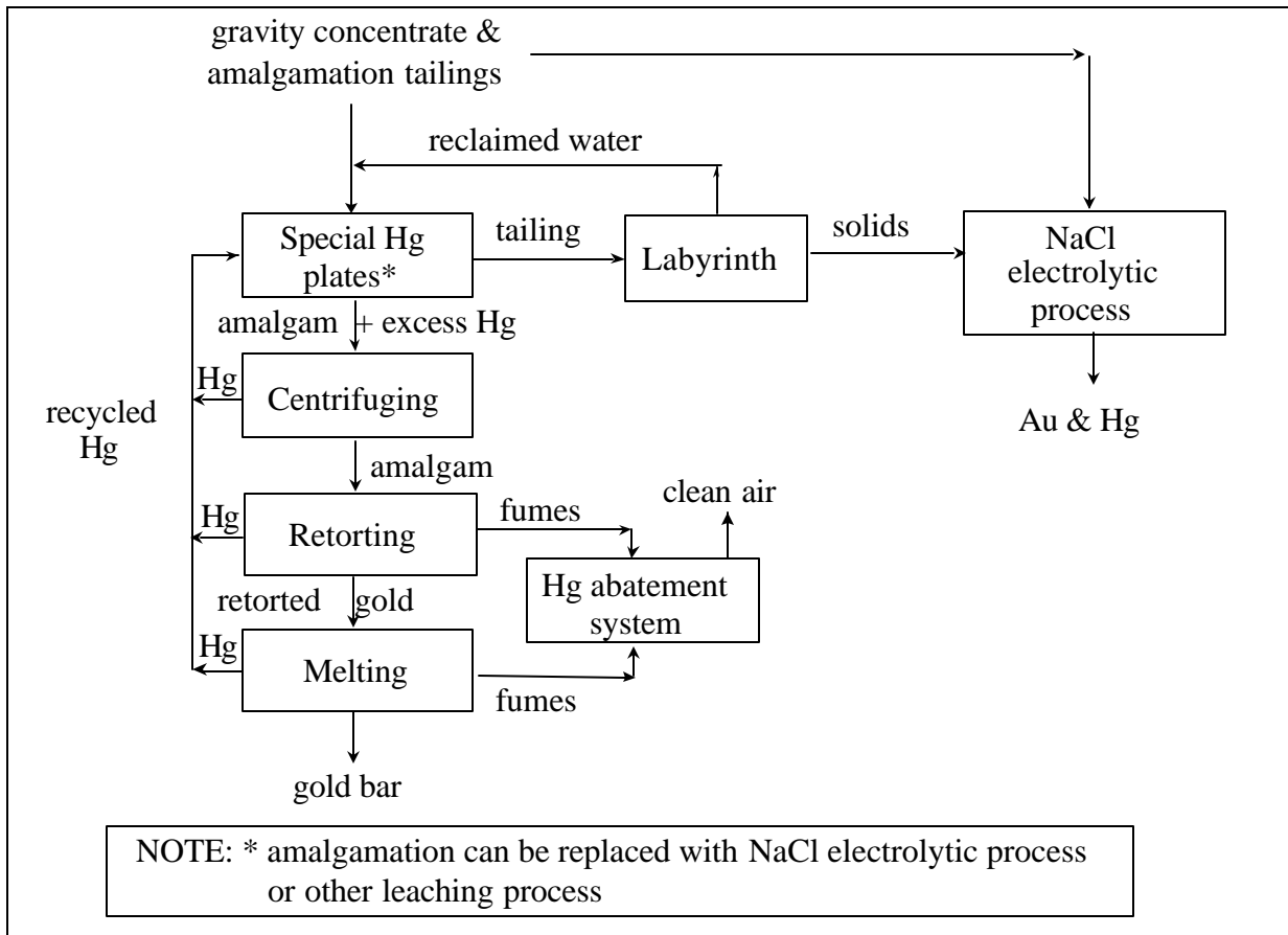
Fig. 6 - Steps in a UNECA Processing Center
